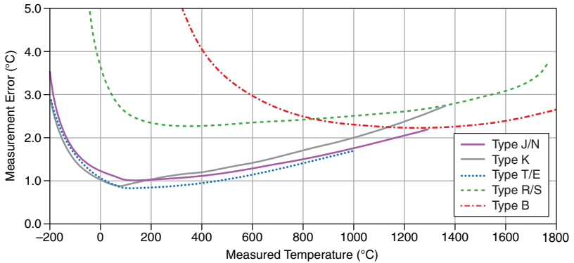
Figure 5. TB-9212 with Screw Terminal Thermocouple Error Maximum (High-Resolution, Best 50/60 Hz Rejection), -20 °C to 70 °C
